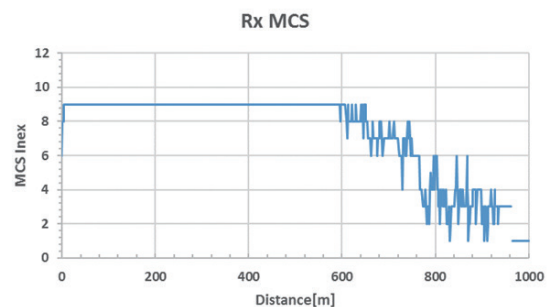
b : Dependence of MCS index on distance.
