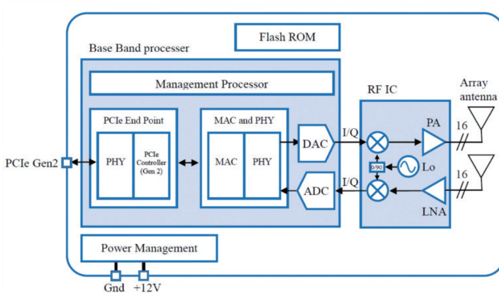
Fig. 2. Functional Block diagram.
