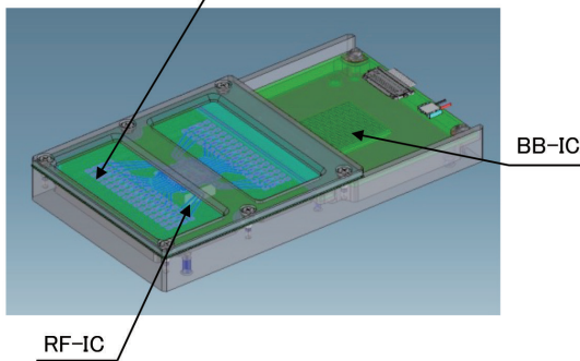
Fig.1. A 60 GHz wide-band communication module.
