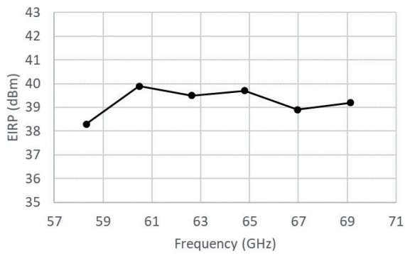
Fig.4. Frequency characteristics of EIRP.
