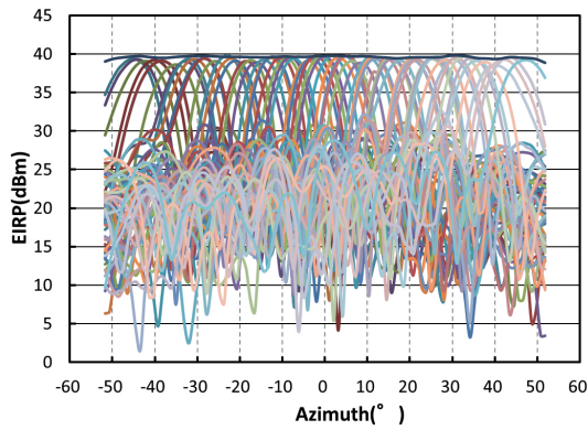
Fig. 3. Beamforming characteristics.
