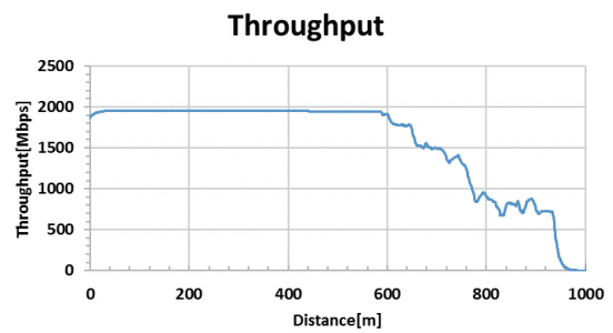
a : Dependence of throughput on distance.
